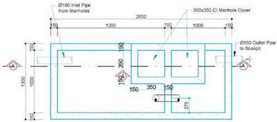
Plan of Septic Tank 5 Users
